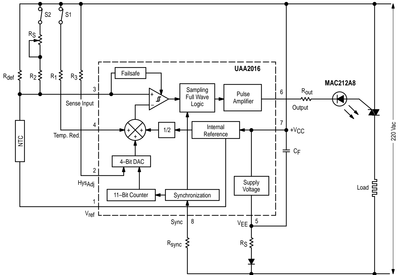
Figure 1. Application Schematic
